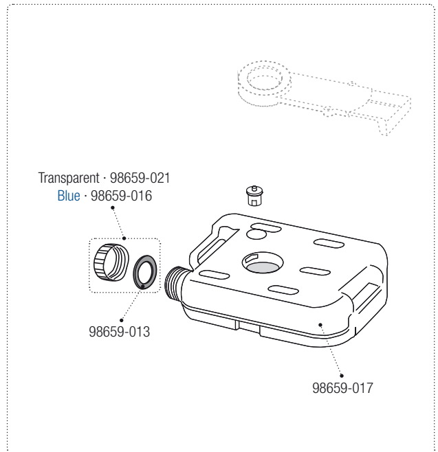
Bi-Pot 1513
